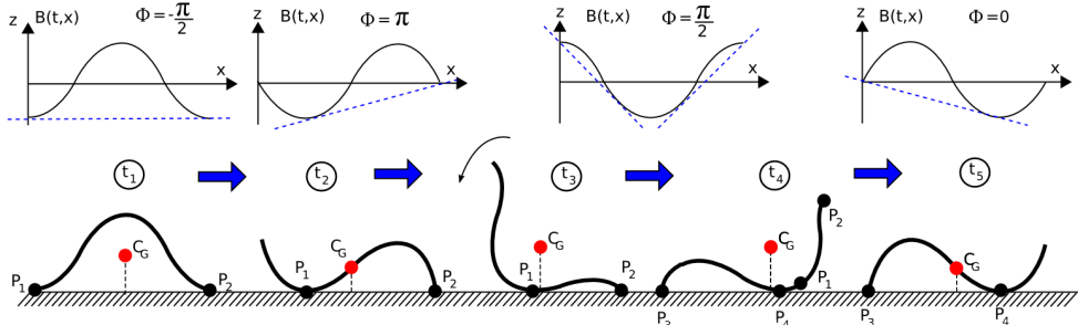
Fig 4.1. Stability of a pitch-connecting robot when its body wave is one ( k=1 )
