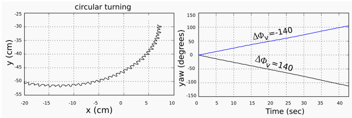
Fig. 6.7. Experimental results for the turning gait
