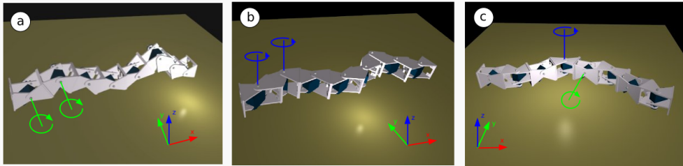
Fig 2.3. Different connections for a snake robot. (a) Pitch connection. (b) Yaw connection. (c) Pitch-yaw connection.
