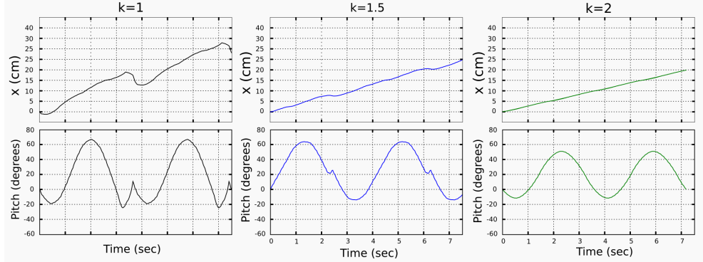
Fig. 6.4. Stability condition experiments for the pitch-connecting modular robot.
