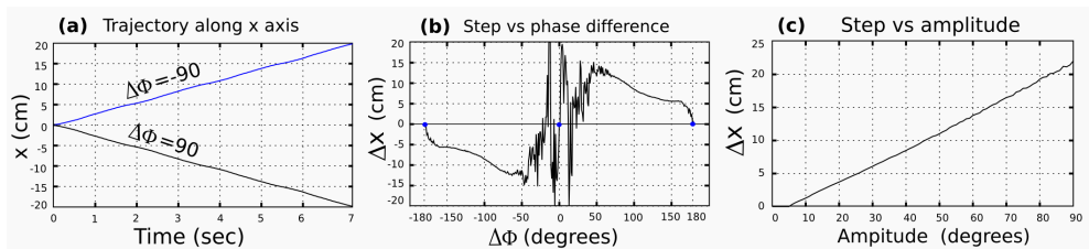
Fig. 6.3. Experiments for the Locomotion in 1D of an 8 module pitch-connecting robot.
