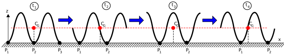
Fig 4.3. Stability of a pitch-connecting robot when its body wave has the value of two( k=2 )
