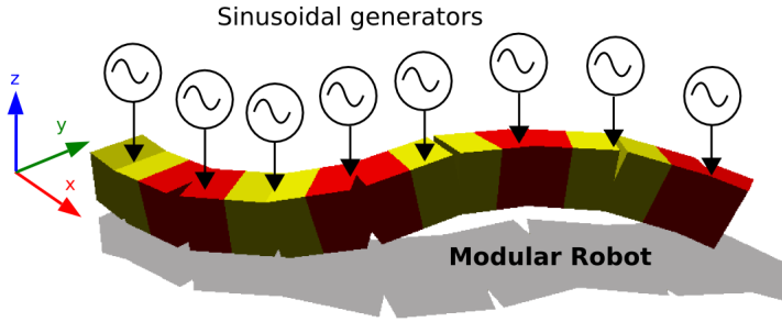
Fig 3.1. Control approach for the locomotion of pitch and pitch-yaw connecting modular robots.
