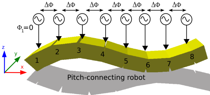
Figure 6. Control of a pitch-connecting modular robot using solution space H1
