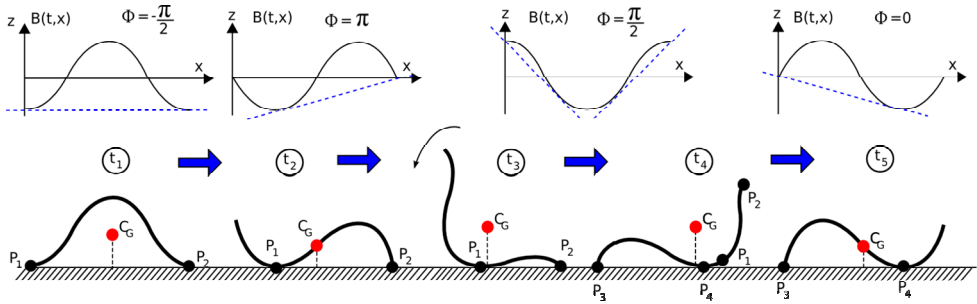
Figure 10. Stability of a pitch-connecting robot when its body wave is one ( k=1 )
