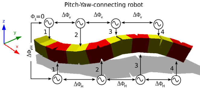
Figure 7. Control of a pitch-yaw-connecting modular robot using solution space H2
