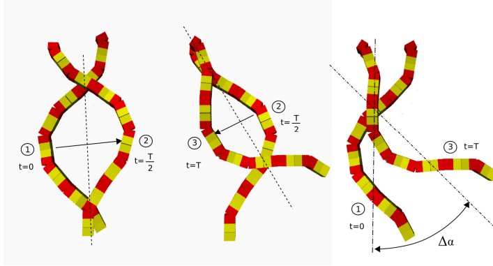
Figure 17. A pitch-yaw connecting robot performing the rotating gait with kh=1
