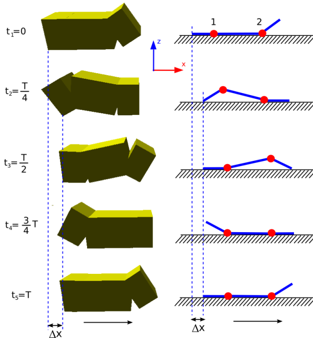
Figure 14. Locomotion of the pitch-pitch (PP) minimal configuration
