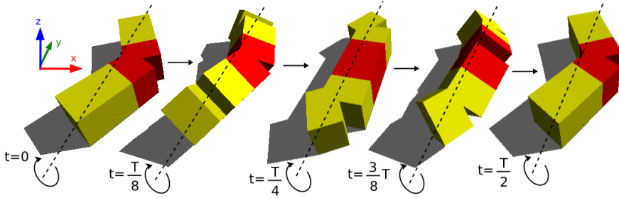
Figure 20. The minimal configuration pitch-yaw-pitch (PYP) performing the rolling gait
