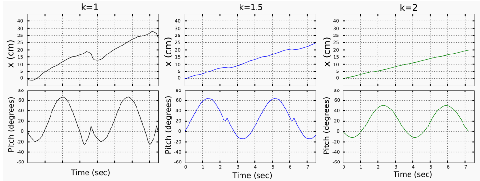
Figure 25. Stability condition experiments for the pitch-connecting modular robot
