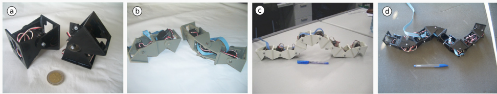
Figure 23. The four robot prototypes built. (a) Y1 modules used to built the robot. (b) The two minimal configurations: PP and PYP. (c) An eight module pitch-connecting modular robot. (d) Pitch-yaw-connecting modular robot with eight modules
